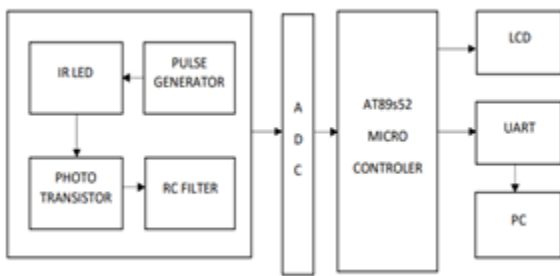
Fig. 1. Block diagram of non invasive glucose monitoring device
