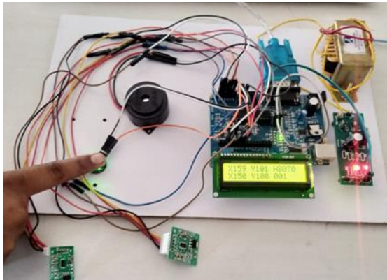
Fig. 9. Final prototype of IoT-based fetal monitoring system for prenatal care
